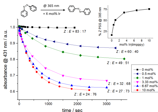
Figure 6. Catalytic reductive Z \rightarrow E isomerization of parent azobenzene 1 triggered by photoinduced electron transfer from an iridium complex (\text{Ir}(\text{dmppy})_3) : Upon addition of catalytic amounts of \text{Ir}(\text{dmppy})_3 to the Z -rich PSS mixture (containing 83% of Z -1) and subsequent irradiation at 365 nm, the amount of E isomer in the PSS is substantially improved (inset, top right) while also the isomerization rate is dramatically increased.
